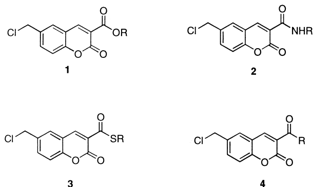
Figure 1. Chemical structures of 6-chloromethylcoumarin esters (1), amides (2), thioesters (3) and ketones (4).
