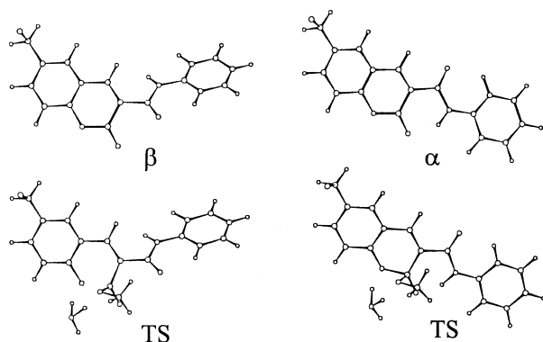
Figure 7. The two minimum conformations of the amide and their respective geometries at the transition state during the reaction with the couple methanol–water.
