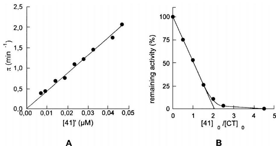
Figure 3. Inactivation of \alpha -CT by compound 41 at pH 7.5 and 25 °C. A. Determination of the constant k_i/K_i by the progress curve analysis. Plot of \pi versus [I] . B. Determination of the partition ratio. Plot of the remaining activity (%) at infinite time versus [I]_0/[E]_0 .
