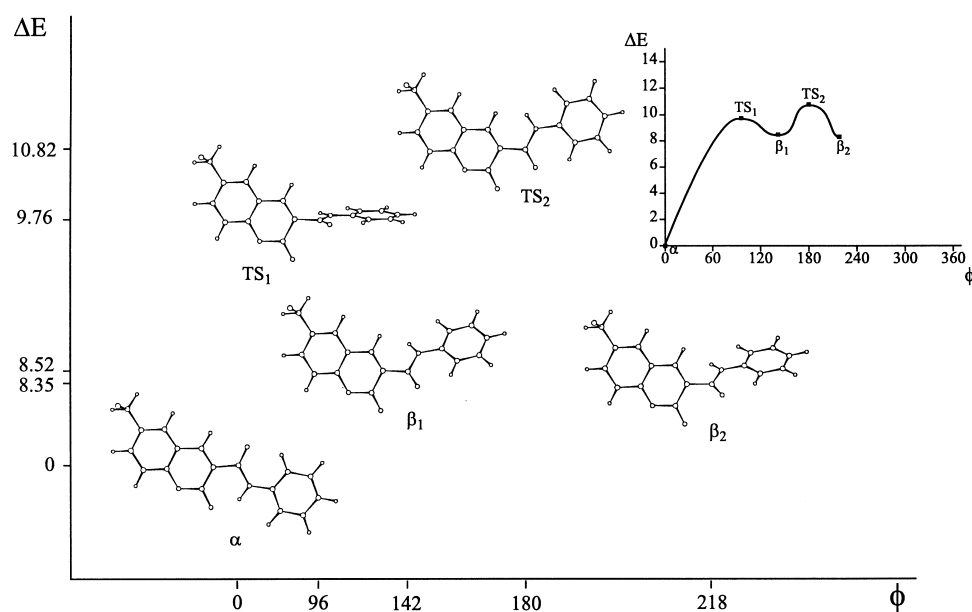
Figure 5. Conformational study of the amide 38 .
