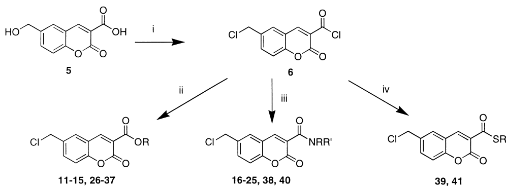
Scheme 1. Reagents: (i) \text{SOCl}_2 ; (ii) \text{ROH} /pyridine/dioxane; (iii) \text{RR}'\text{NH} /pyridine/dioxane; (iv) \text{RSH} /pyridine/dioxane.
