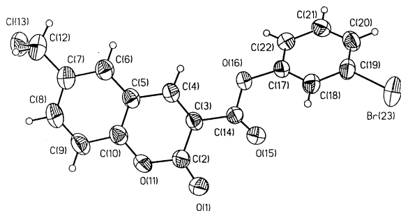
Figure 4. ORTEP representation of X-ray structure of 30 .
