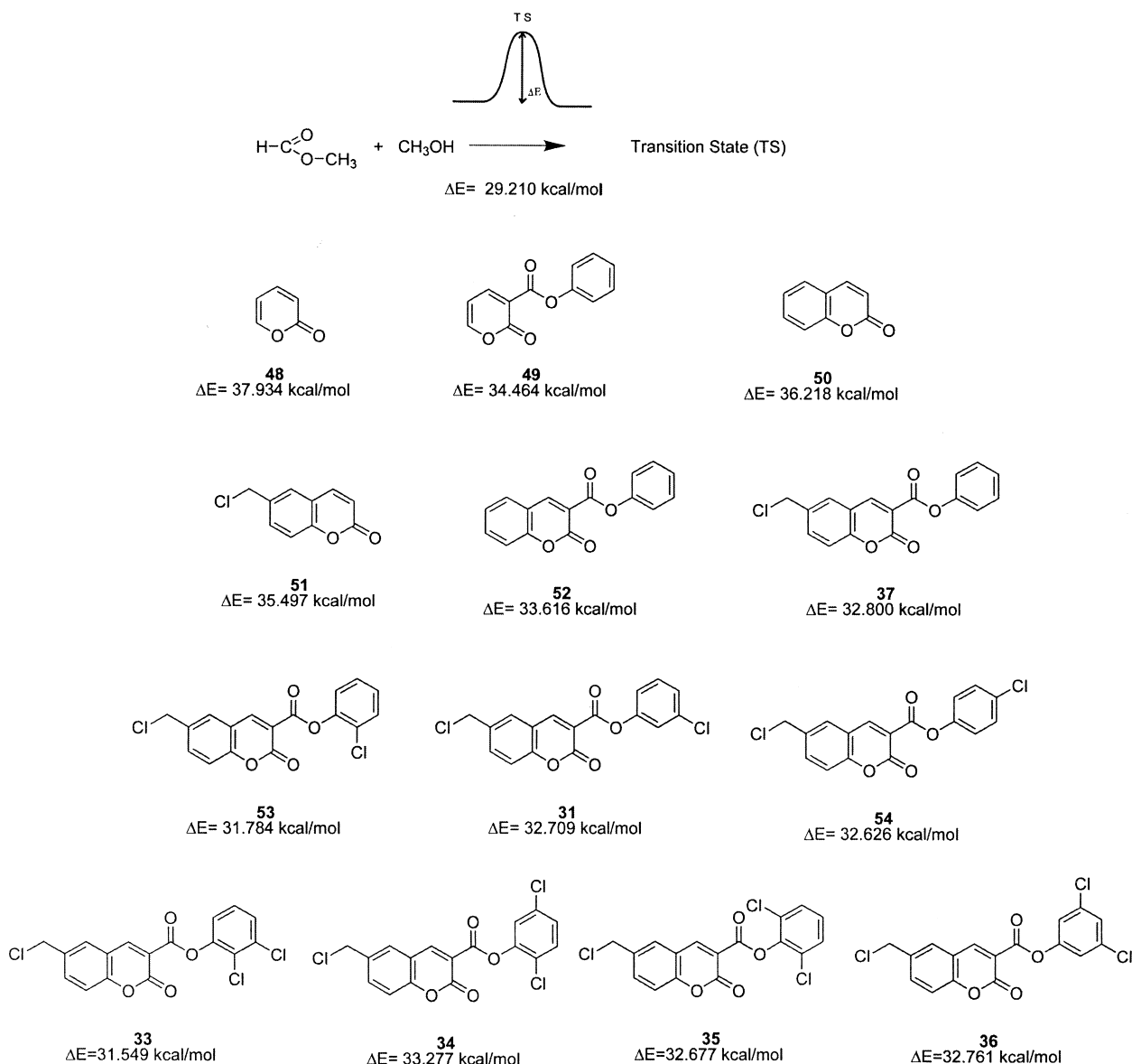
Figure 6. Intrinsic reactivity of the nucleophilic reaction.
