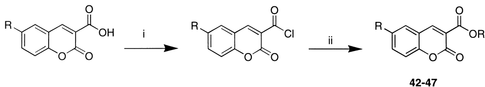
Scheme 3. Reagents: (i) \text{SOCl}_2 ; (ii) \text{ROH} /pyridine/dioxane.
