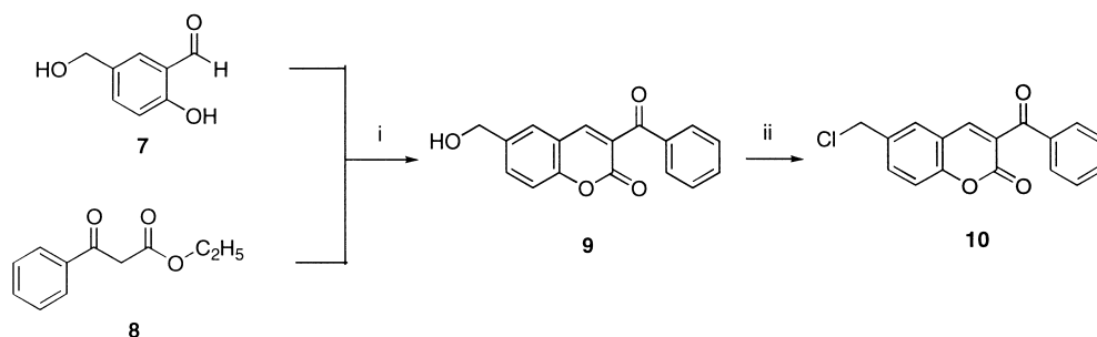
Scheme 2. Reagents: (i) piperidine/EtOH; (ii) \text{SOCl}_2 .
