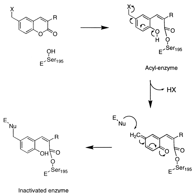
Figure 2. Postulated mechanism for the inactivation of \alpha -chymotrypsin by coumarinic derivatives.
